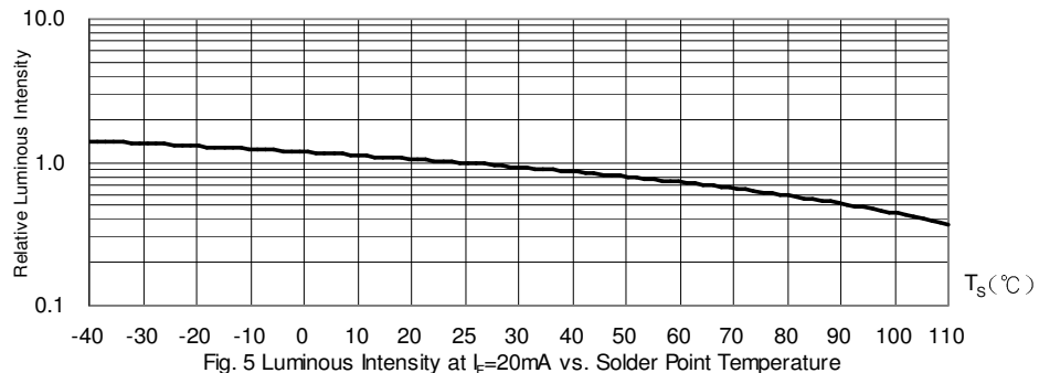
Fig. 5 Luminous Intensity at I_F=20\text{mA} vs. Solder Point Temperature
