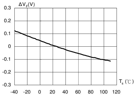
Fig. 3 Relative Forward Voltage vs. Solder Point Temperature \Delta V_F = V_F - V_F(25^\circ\text{C}) = f(T_s) ; I_F = 20\text{mA}
