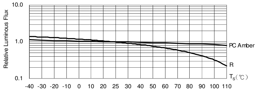
Fig. 5 Luminous Flux at I_F=140\text{mA} vs. Solder Point Temperature
